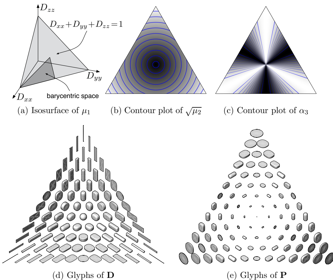
Figure 5.5. The space of orientation changes, as represented by \mathbf{P} , is reduced from three to two dimensions when eigenvalue skewness \alpha_3 is at extremum, and is reduced to zero dimensions when eigenvalue variance \mu_2 is zero.
