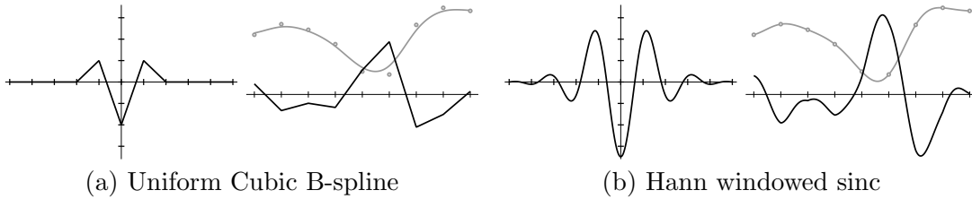
Figure 2.4. Effect of second derivative kernel choice (left) on second derivative measurement result (right), for two of the kernels used in Figure 2.2.
