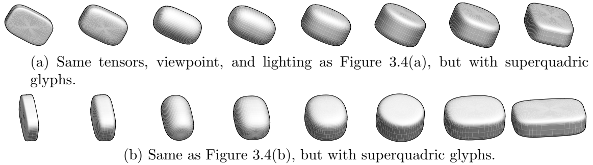
Figure 3.8. Superquadrics convey shape differences more reliably than ellipsoids ( \gamma = 3 ).
