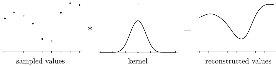
Figure 2.1. Convoluting discretely sampled values with a continuous kernel generates a continuous signal. Note that the mathematical definition of convolution involves replacing the discrete sample values with scaled Dirac delta functions in the continuous domain.
