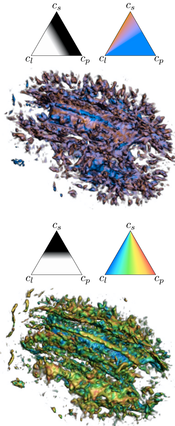
Figure 6.2. Examples of barycentric color maps and resulting renderings.
